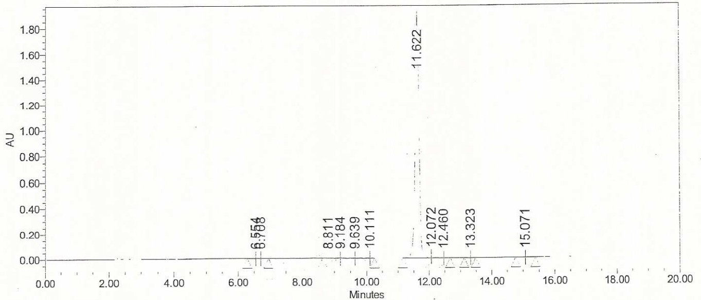
Auto-Scaled Chromatogram
